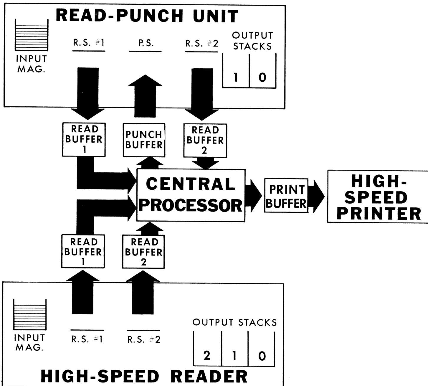
Figure 3. Buffer Operation
