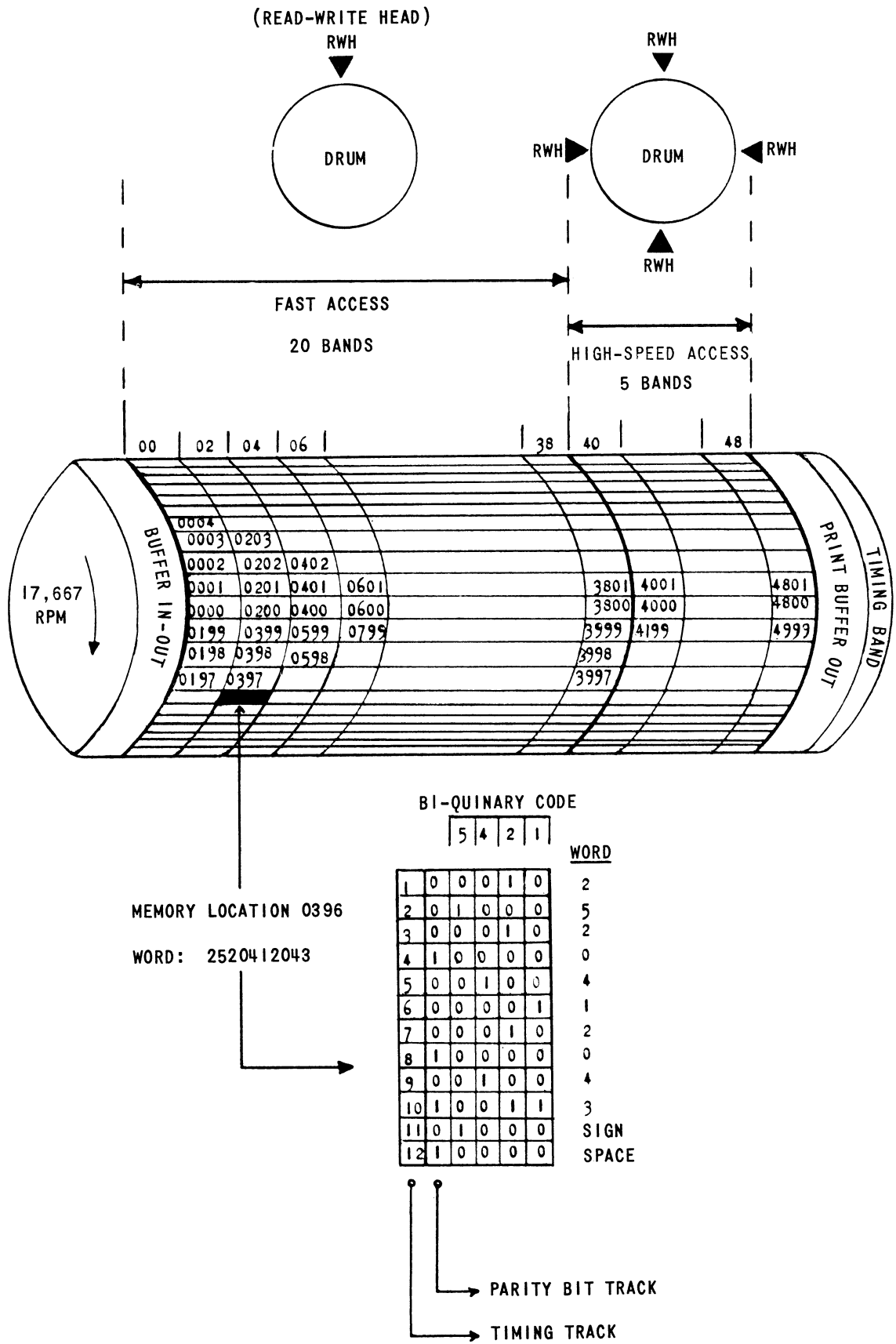
Figure 1. Magnetic Storage Drum
